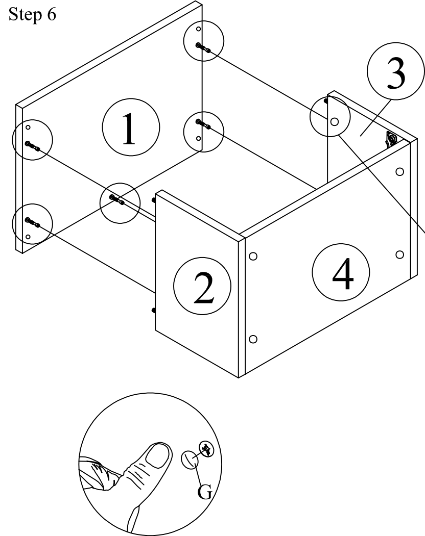
*Attach Minifix Cap as shown.
