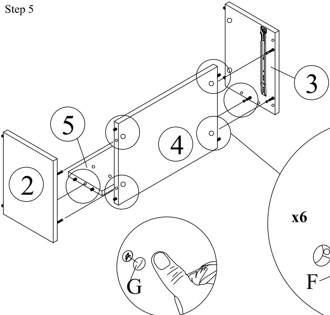
*Attach Minifix Cap as shown.
